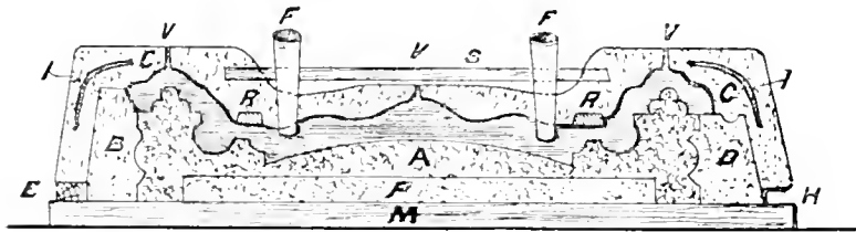
NO. 134.—SECTION OF MOULDING PIECE, WITH JELLY MOULD, PLASTER PICES, AND CASE FOR PROSCENIUM PANEL.
